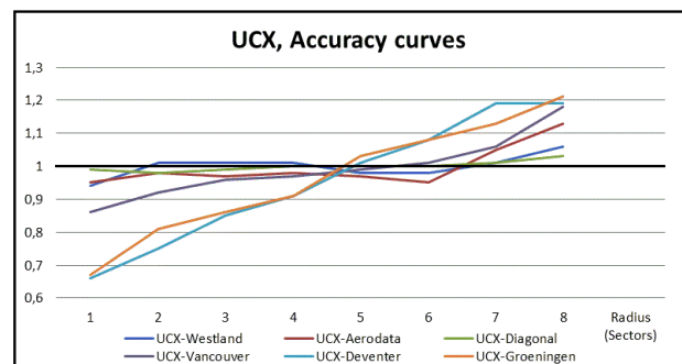
Fig. 3b Accuracy as function of radius for UCX camera types
