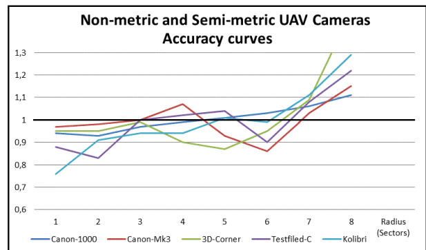
Fig. 6 Accuracy as function of radius Non- and Semi-metric camera types
