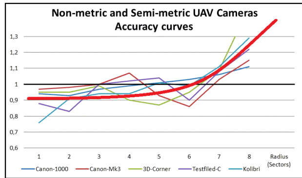
Fig. 11 Accuracy of the Non-metric and Semi-metric camera types with fitted curve
